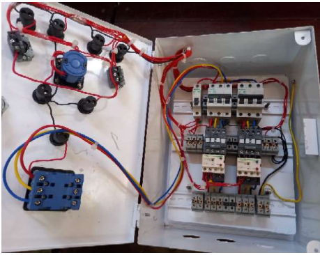
Pump Control
